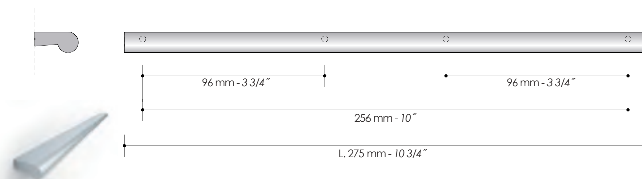
Maniglia per ante piene, vetro acidato o vetro retrolaccato con telaio in alluminio e vetro fumè. Handle for wooden doors, acetated or rear-lacquered glass with aluminium frame and smoked glass doors.
